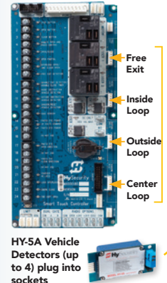
Smart Touch Controller Keypad Smart Touch Controller Board
