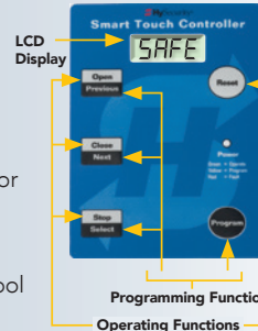
Smart Touch Controller Keypad
