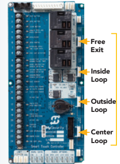
Smart Touch Controller Board
